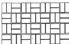
BASKETWEAVE Brick Size 92mm x 197mm
